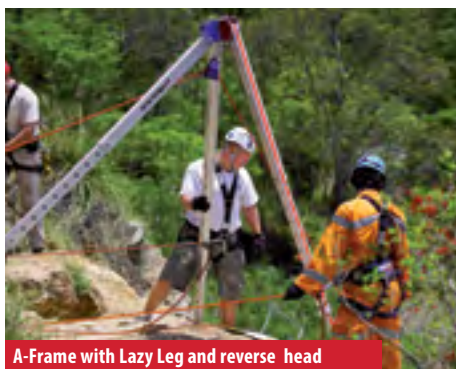
A-Frame with Lazy Leg and reverse head
