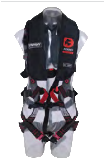
Challenge Pro with integral PFD certified to AS/NZS 4758.1 & AS/NZS 1891.1:2007
